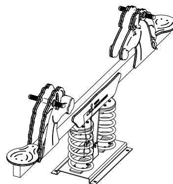
VISTA ISOMÉTRICA ISOMETRIC VIEW
